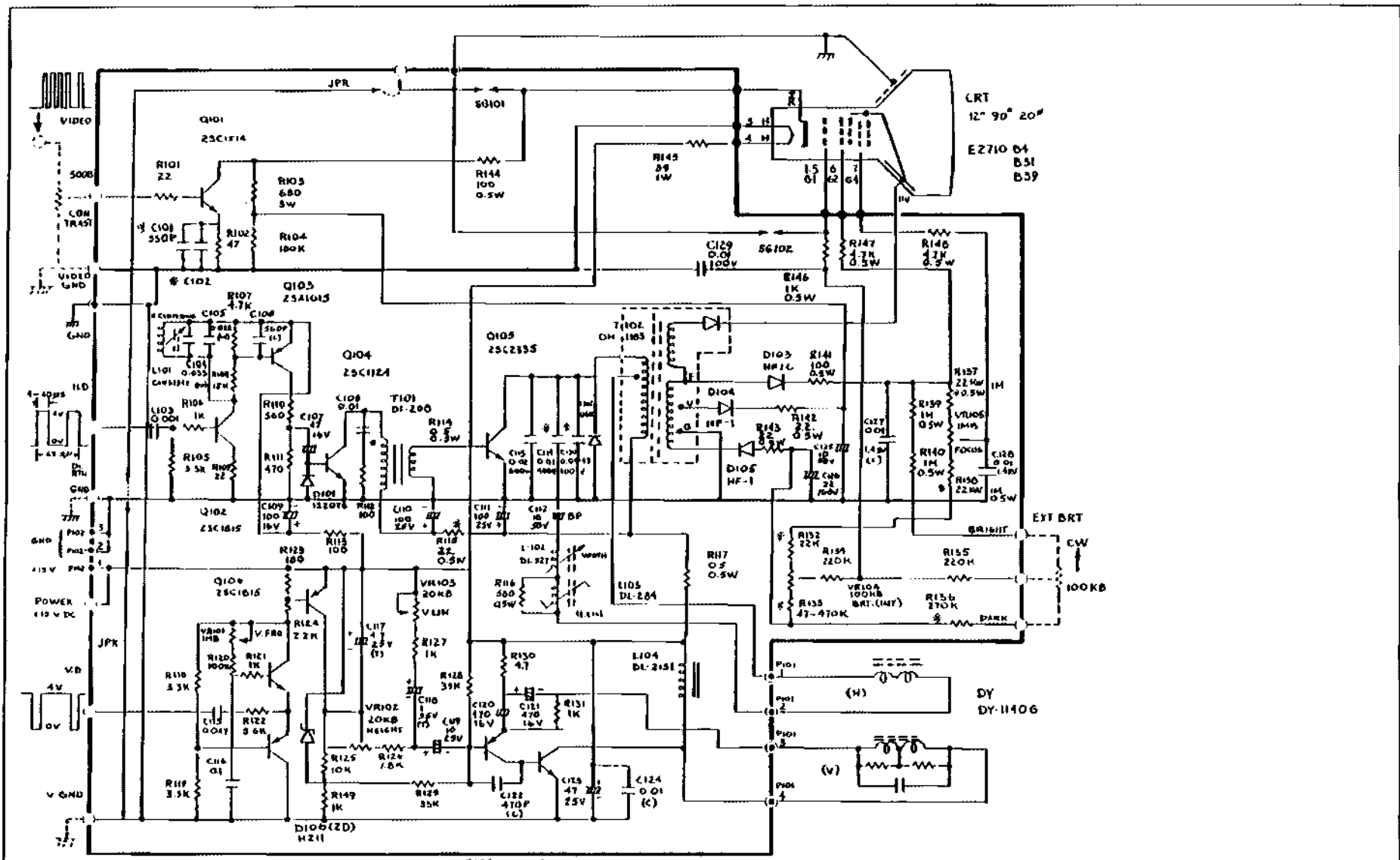
CIQ-12 AND 9 15VDC VERSION CIRCUIT DIAGRAM
