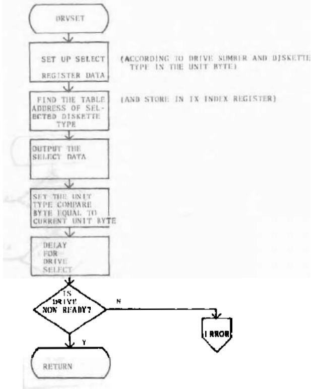
DRIVE SELECTION SEQUENCE FIG 3-3
