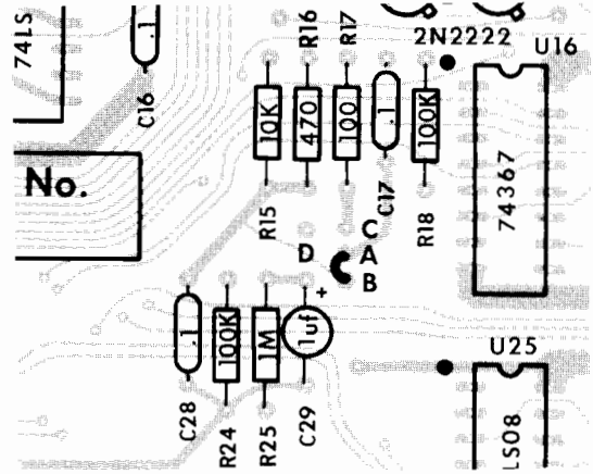
Figure 7. CUTS Jumper
