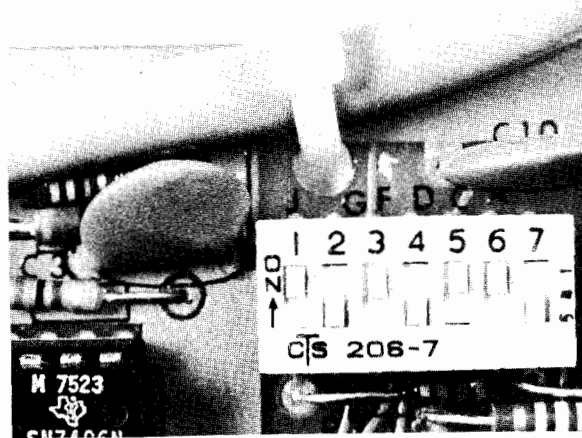
Figure 6 VDM-1 Switches
