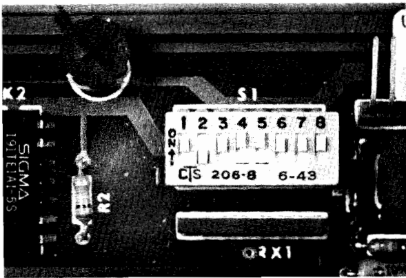
Figure 8. CUTS Switches
