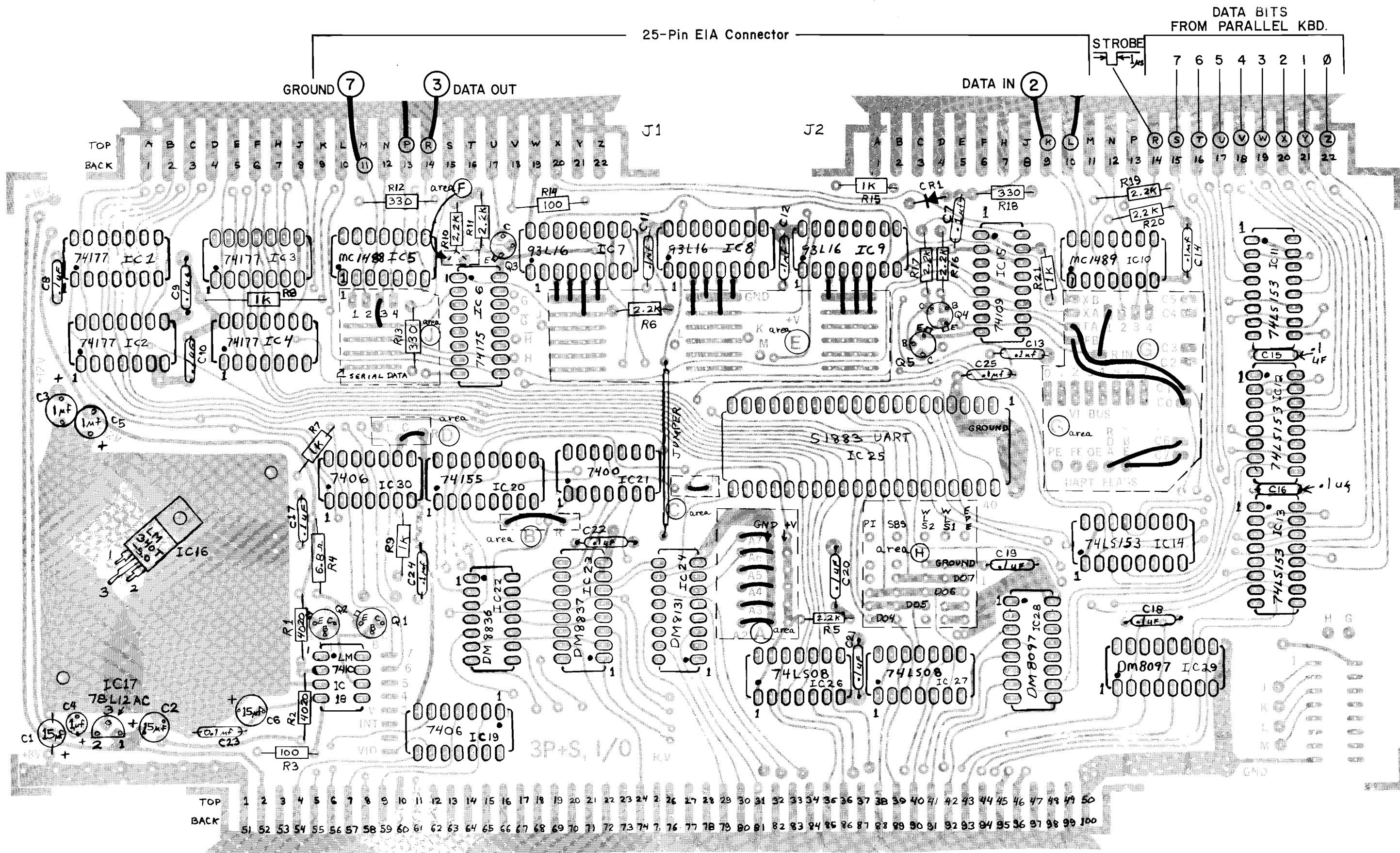
Figure 3. Jumpering 3P+S for Keyboard Console and RS232-C Serial Interface
