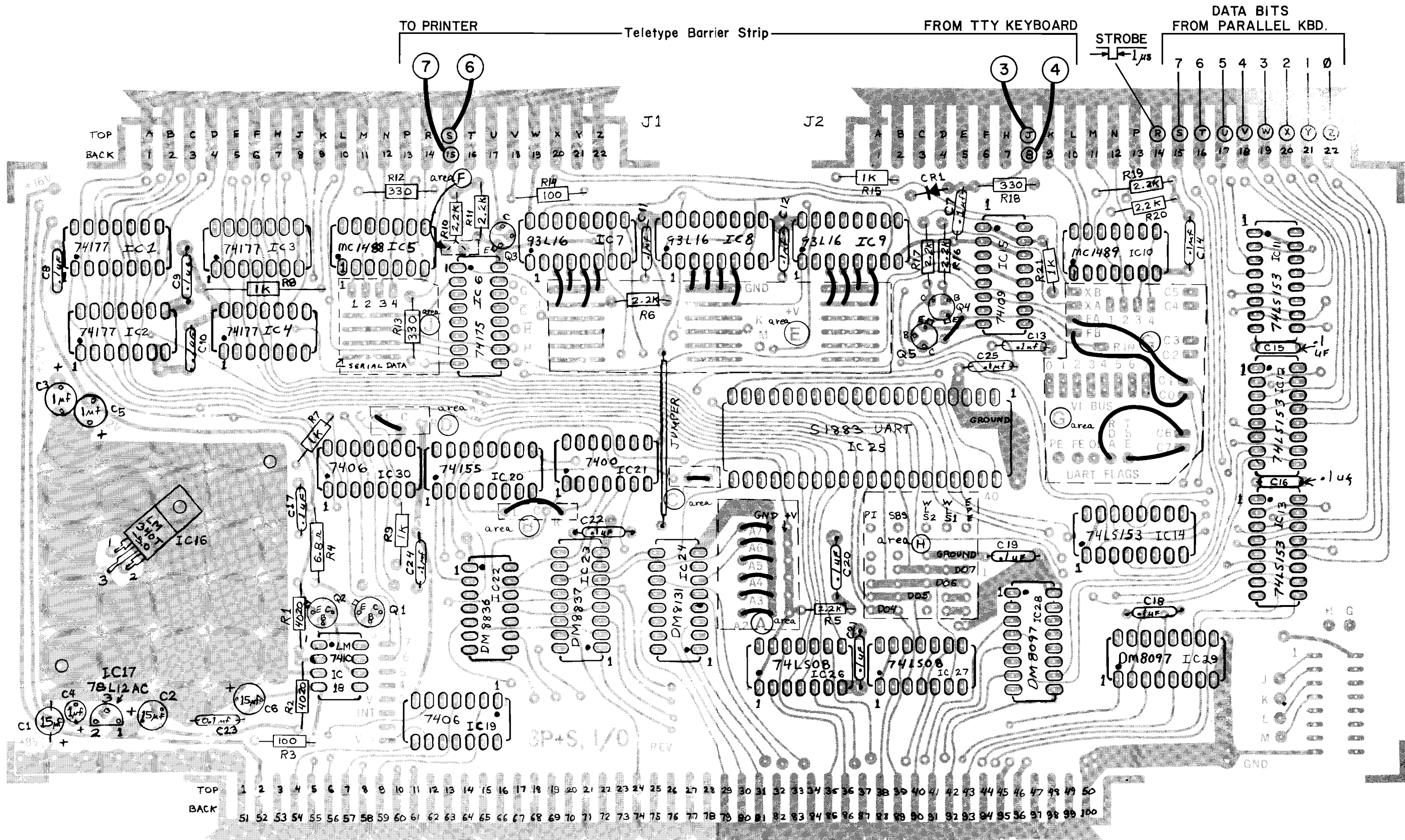
Figure 4. Jumpering 3P+S for Keyboard Console and Current Loop Serial Interface
