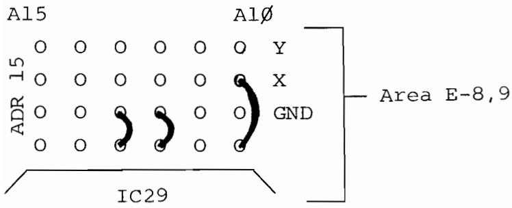
Figure 5. VDM-1 Jumpers
