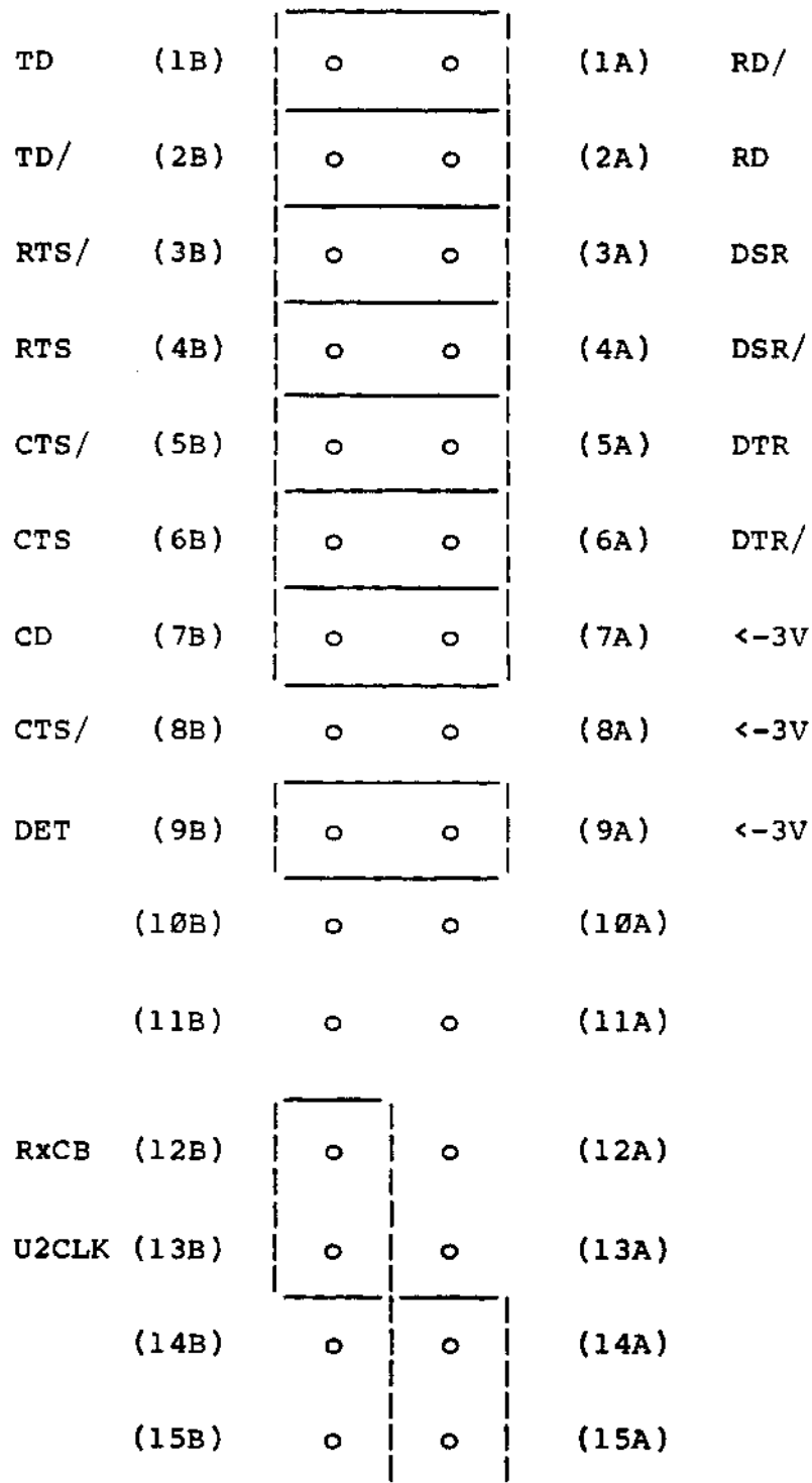
Figure D-6. Factory jumper settings for JPC
