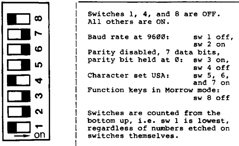
Figure 1-6: MDT-60 Setup Switches, Properly Set for MD-11
