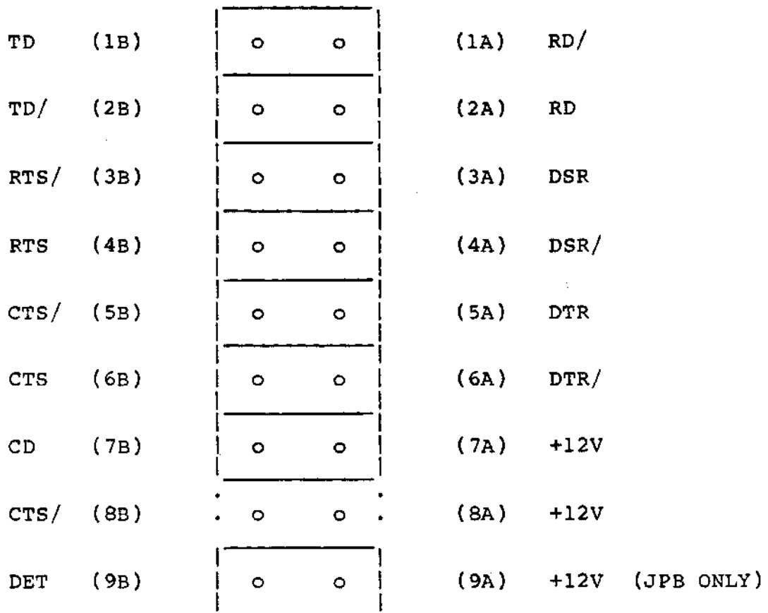
Figure D-5. Factory Jumper Settings for JPA/B
