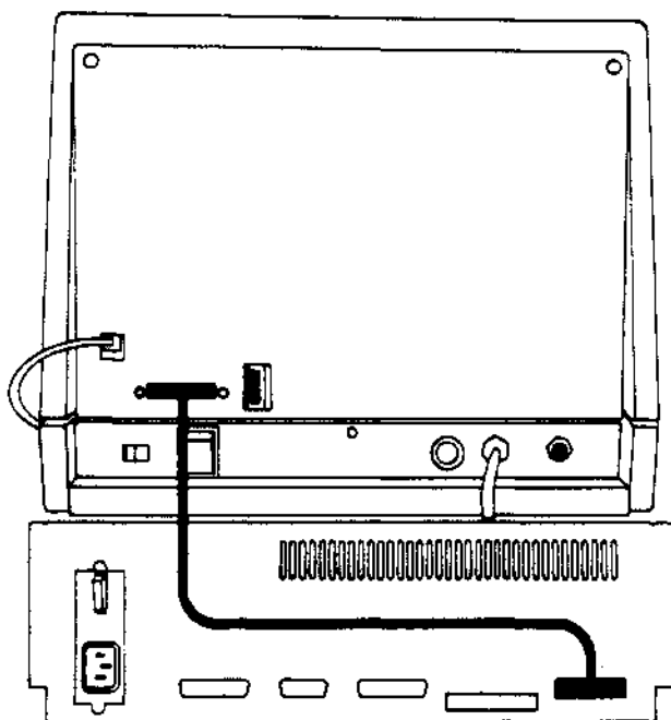
Figure 1-1: Terminal Cable Connection (MDT-68 Terminal shown)
