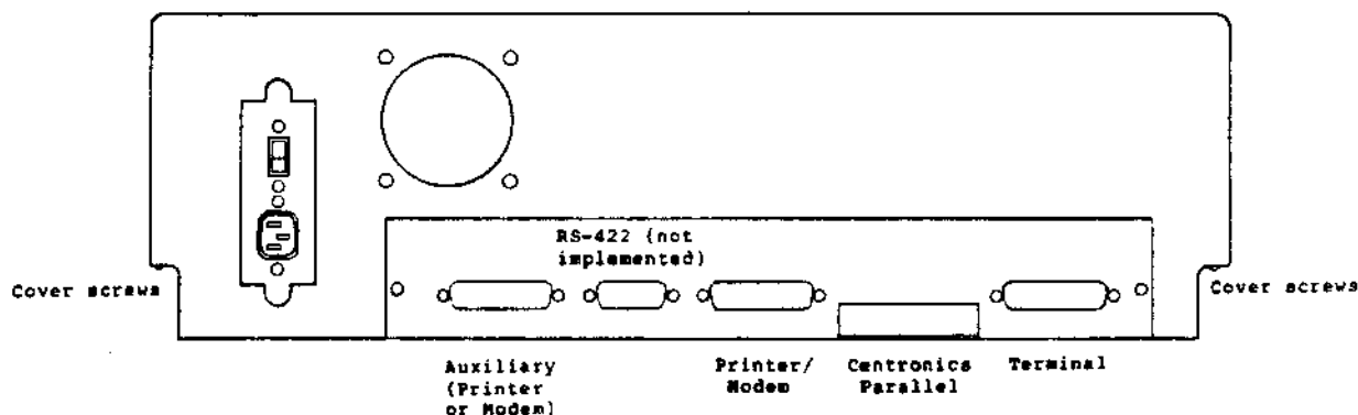
Figure D-1. MD-11 peripheral connectors
