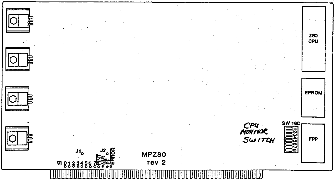
CPU PCB
