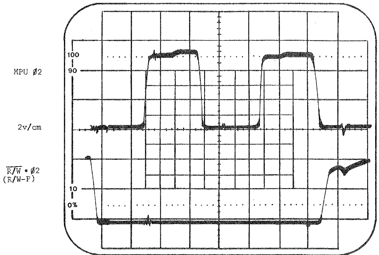
READ/WRITE PRIME During WRITE Cycle
