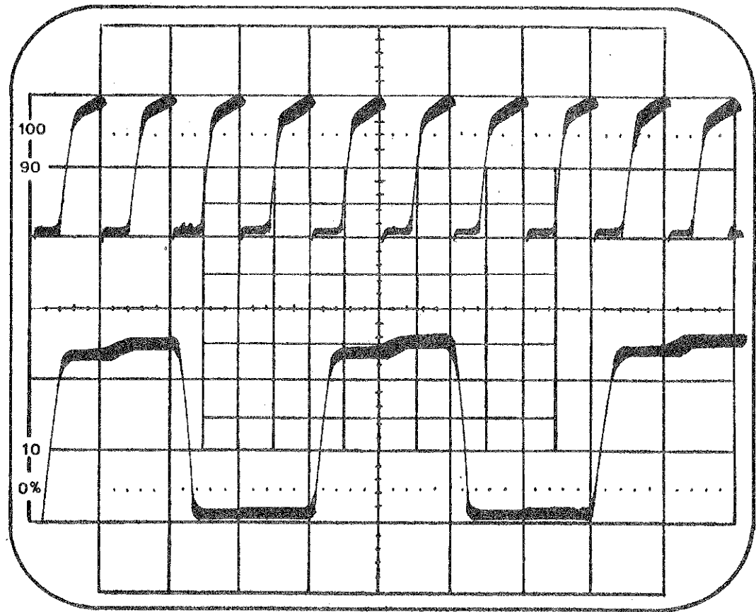
2 MHz Clock and MPU \phi 2 Clock
