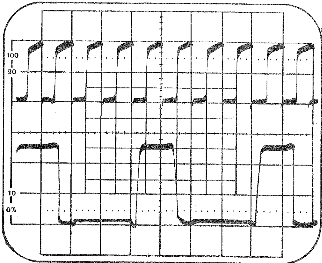
2 MHz Clock and MPU \phi 1 Clock
