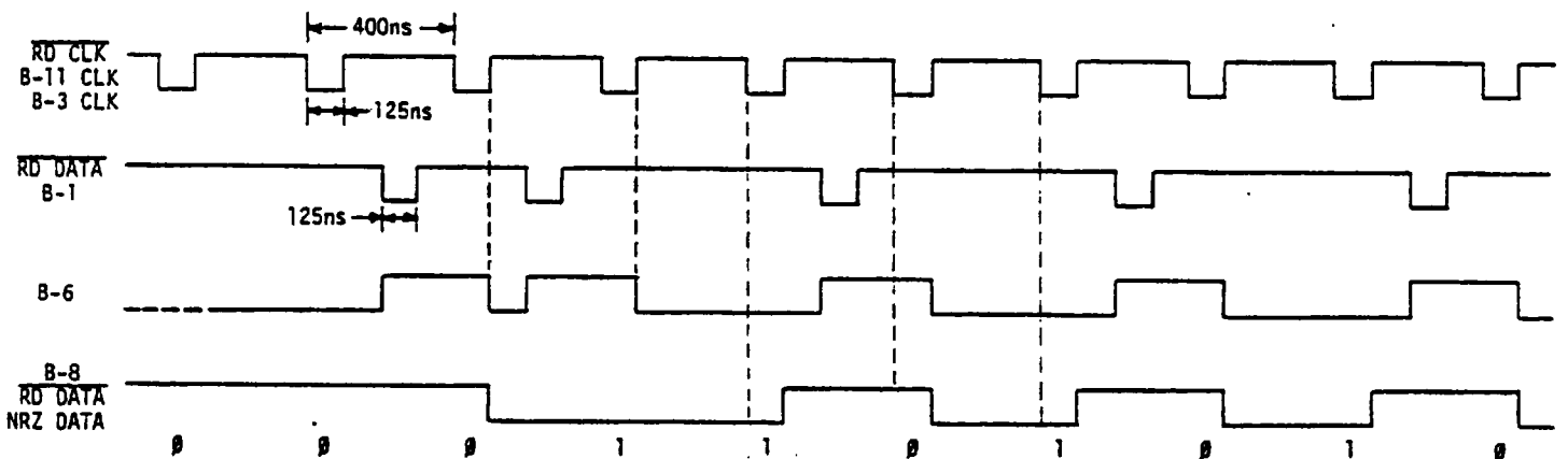
Figure 4-6. Read Data Timing
