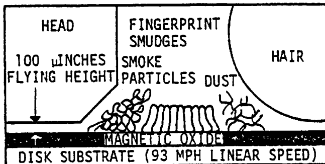
Figure 3-1. Head Sensitivity
