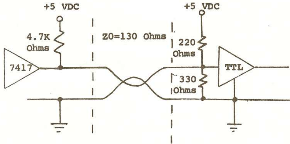
FIGURE 5 LINE DRIVERS AND RECEIVERS
