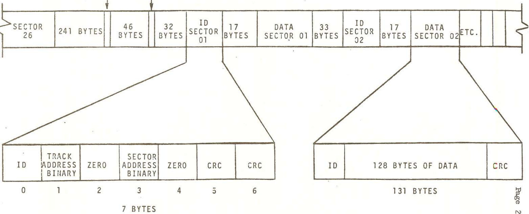
FIGURE 4. IBM DATA FORMAT
